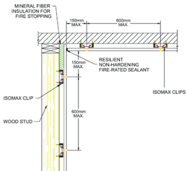
RESILIENTLY MOUNTED WALL & CEILING
